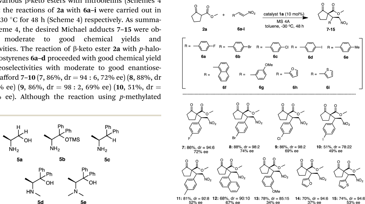
Scheme 3 Substituted amino alcohol organocatalysts 5a–e .
