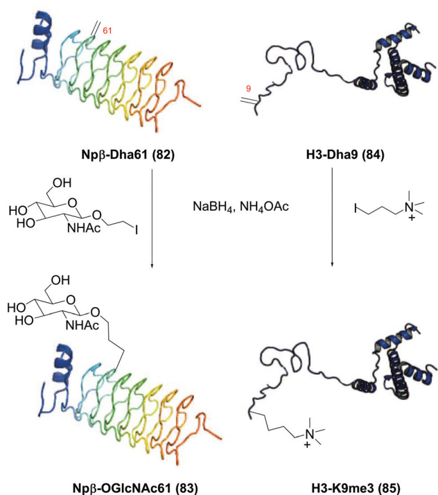
Scheme 21 Protein functionalization with C-radicals by Davis et al. 74a
