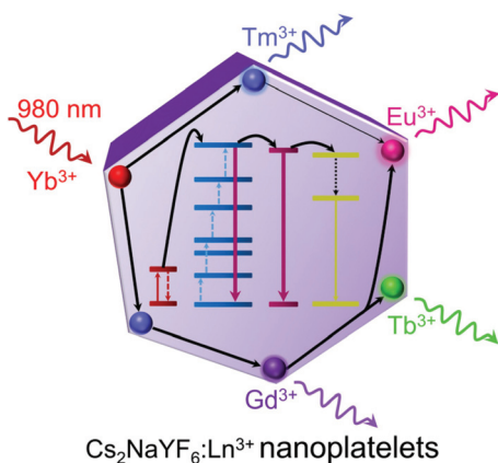
Scheme 1 Schematic illustration of \text{Cs}_2\text{NaYF}_6:\text{Ln}^{3+} NPs with highly efficient multiphoton UC emission upon 980 nm excitation.
