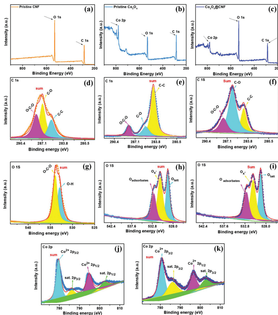
Fig. 3 (a–c) XPS survey spectra of pristine CNF, pristine Co 3 O 4 nanoparticles and 1D Co 3 O 4 @CNF hybrid; (d–f) C 1s binding energy region and (g–i) O 1s binding energy region and (j and k) Co 2p binding energy region for the respective samples.
