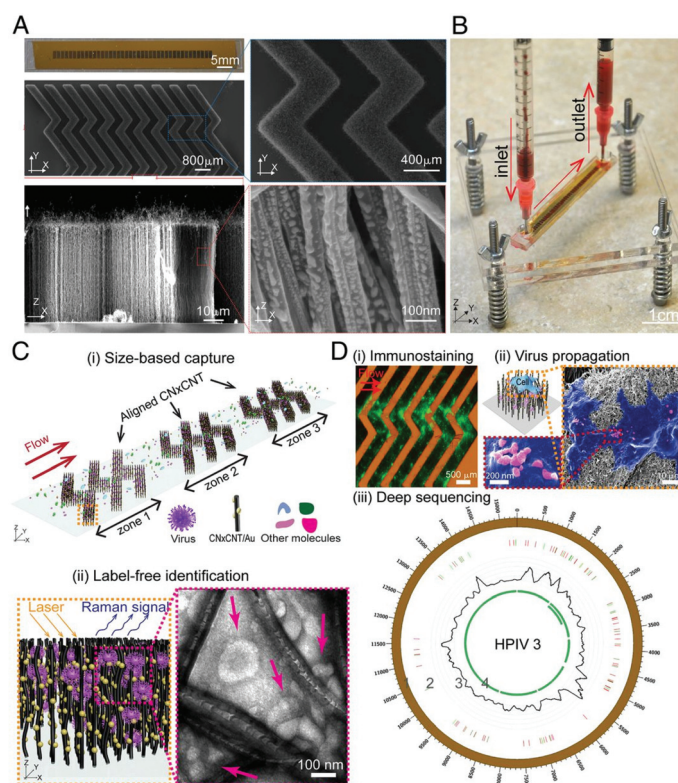
Fig. 10 Schematic of the working principle of VIRRION platform, including (A) images of aligned CNTs decorated with gold nanoparticles and (B) assembled VIRRION device, (C) illustration of virus capture and label-free Raman identification, and (D) on-chip analysis and enrichment of virus for NGS. Reprinted with no changes from ref. 122, image licensed under http://creativecommons.org/licenses/by/4.0/ .
