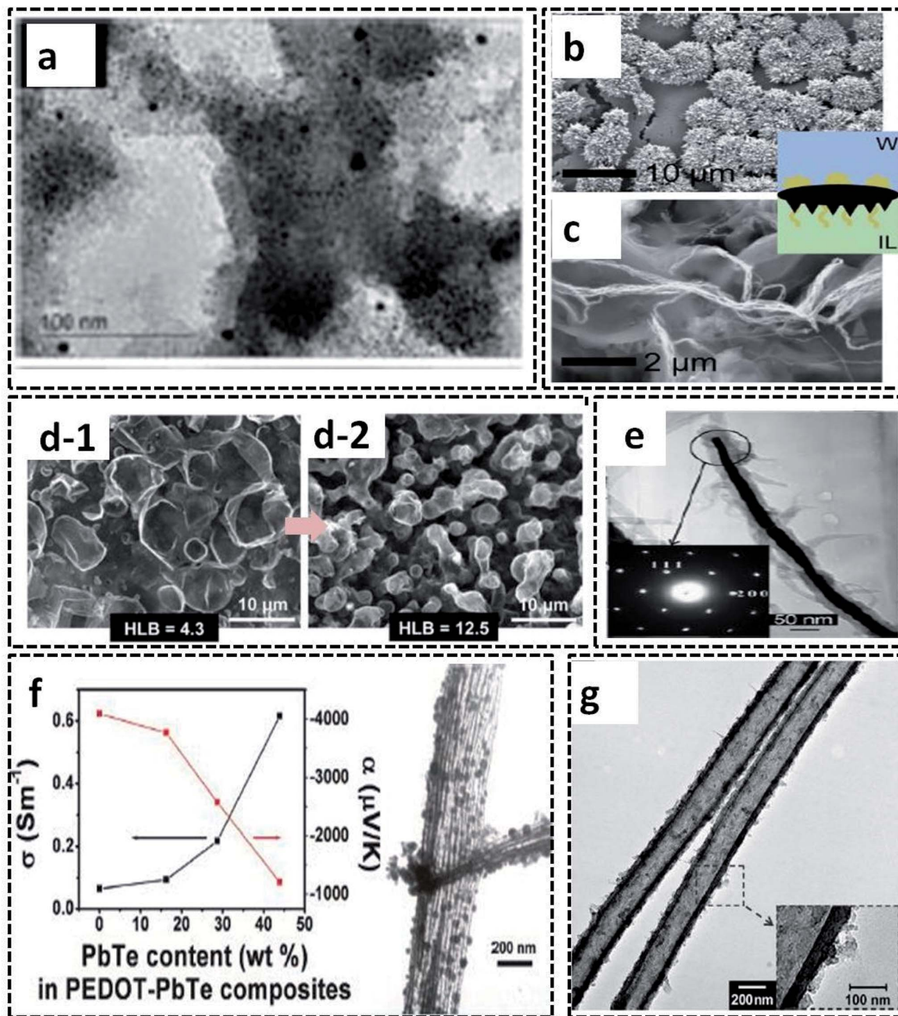
Fig. 10 (a) TEM images of the PTh/Au film. Reprinted from ref. 102, Copyright (2018), with permission from Elsevier. SEM images of (b) microrochin and (c) dendrite-like fiber shapes of the PTh/Au composite prepared by ionic liquid/water interfacial polymerization. Reprinted with permission from ref. 21. Copyright (2018) American Chemical Society. (d) SEM images of PPY synthesized by water/chloroform interface-assisted polymerization in the presence of a surfactant mixture (Span 80 and OP 10). The transformation of the morphology from a ruptured vesicle type to coral type is shown in the figure with an arrow. Reprinted from ref. 104, Copyright (2018), with permission from Elsevier. (e) TEM image of PEDOT/Au nanocable with inset showing the SAED pattern of the highly crystalline Au. Reprinted with permission from ref. 2. Copyright (2007) American Chemical Society. (f) TEM image of the PEDOT-PbTe composite tubes showing thermoelectric property. Reprinted with permission from ref. 105. Copyright (2011) American Chemical Society. (g) The TEM image of the 1-D PEDOT nanotubes prepared by water in oil micro-emulsion interfacial polymerization method. Reproduced with permission under a Creative Commons CC-BY License from ref. 106. Copyright 2007 John Wiley and Sons.
