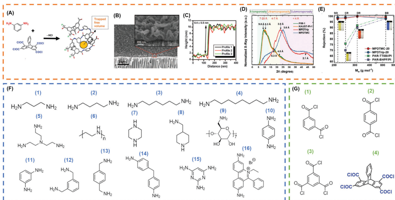
Fig. 8 (A) Reaction between MPD and triptcene-1,3,6,8-tetraacetyl chloride (Trip) to form a PA layer with high free volume. 73 Copyright 2020, WILEY-VCH. (B) SEM imaging of MPD/TMC TFC suggesting improved surface area due to crumpled surface. 125 (C) AFM imaging of MPD/TMC films on silicon wafer suggesting PA selective layer is less than 10 nm. 125 Copyright 2015, Science. (D) Comparison of XRD patterns of PA layers derived from MPD/TMC and MPD/Trip. 73 (E) Rejection profile of various dyes in methanol for eclectic membranes (SO = Sudan Orange, 216 \text{g mol}^{-1} , CR = Chrysoidine G, 249 \text{g mol}^{-1} , DR = Disperse Red, 314 \text{g mol}^{-1} , BB = Brilliant Blue R, 826 \text{g mol}^{-1} ). 73 Copyright 2020, WILEY-VCH. (F) Frequently used amines for IP: (1) propanediamine, (2) butanediamine, (3) hexanediamine, (4) octanediamine, (5) tris(2-aminoethyl)amine, (6) PEI, (7) piperazine, (8) 4-(aminomethyl)piperidine, (9) amino- \beta -cyclodextrin, (10) p -phenylenediamine, (11) MPD, (12) m -xylenediamine, (13) p -xylenediamine, (14) 4,4'-diaminodiphenylmethane, (15) 2,4,6-triaminopyrimidine, and (16) ethidium bromide. (G) Frequently used acyl chloride for IP: (1) isophthaloylchloride, (2) terephthaloyl chloride, (3) TMC, and (4) trip.
