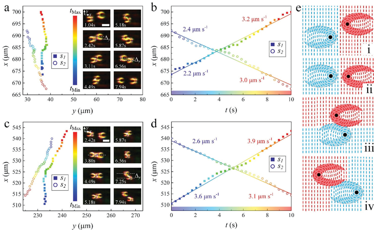
Fig. 7 Dynamic interactions between two swallow-tail solitons. (a and c) Trajectories of two solitons colliding with each other. The color bar represents the elapsed time. t_{Min} = 0 s, t_{Max} = 10 s, time interval \Delta t = 0.345 s. Insets are time series of polarizing micrographs of the solitons during the collisions, scale bars 10 \mu\text{m} . (b and d) The corresponding time dependences of the x -coordinates of the pairs of solitons corresponding to (a and c), respectively. (a and b) U = 5.6 V, f = 2 Hz, T = 34.8 °C; (c and d) U = 8.0 V, f = 10 Hz, T = 34.0 °C. (e) Schematic layer configurations of the solitons in the collisions. (i, iii and iv) show the time development of two solitons pass through each other ( \Delta y \gg R_c ) corresponding to (a and b); (ii, iii and iv) show the time development of two solitons collide head-on ( \Delta y \leq R_c ) corresponding to (c and d). The blue and red dashed lines represent the SmA layers.
