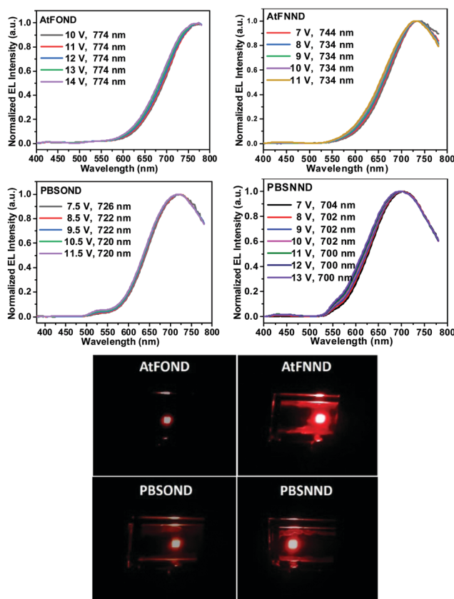
Fig. 8 Top figures: intensity normalized EL spectra AtFOND, AtFNND, PBSOND, and PBSNND NIR OLEDs at varied voltage. Bottom figures: corresponding photographs of each device at \sim 4 –6 V.
