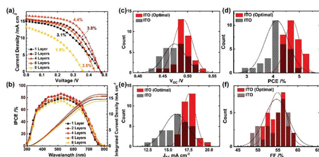
Fig. 3 (a) Representative J-V curves measured under standard one-sun illumination and (b) IPCE spectra of ITO devices with varied layers. (c–f) Statistical histogram of 30 ITO devices each at non-optimal and optimal conditions; all photovoltaic parameters are improved concurrently with minimal spread following optimization.
