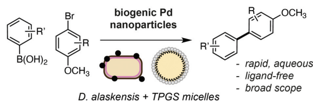
Scheme 1 Approaches to the Suzuki Miyaura cross-coupling reactions in TPGS micelles using chemically synthesised or biogenic palladium nanoparticles.
