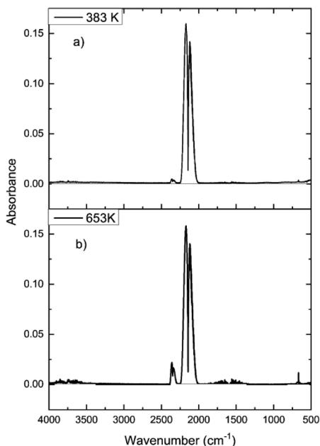
Fig. 11 FTIR spectra for continuous CO dosing over the dried support material (attapulgit) at (a) 383 and (b) 653 K. Flow conditions: CO 5 \text{ cm}^3 \text{ min}^{-1} , N 2 (carrier gas) 54 \text{ cm}^3 \text{ min}^{-1} , and N 2 (diluent post-reactor) 100 \text{ cm}^3 \text{ min}^{-1} .
