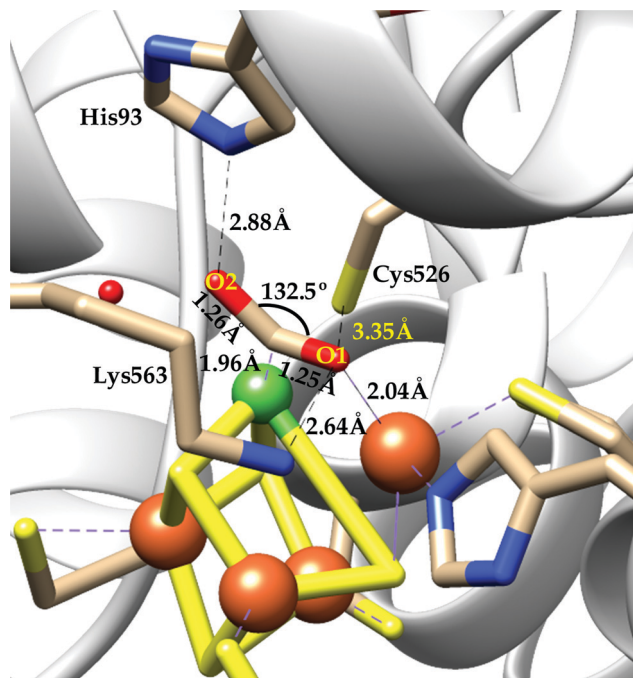
Fig. 2 The structure of ChCODH with \text{CO}_2 ( -600 mV + \text{CO}_2 state; pdb: 3B52). 39
