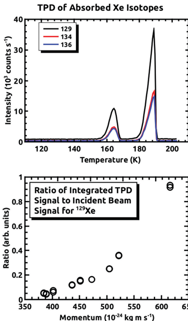
Fig. 3 Top panel: Thermal desorption spectra for the three Xe isotopes taken after a 45 minute exposure of the surface to D 2 O and Xe ( \langle v \rangle = 2.88 \times 10^3 m s -1 ) at \theta_i = 10^\circ , with a linear ramp rate of 10 K min -1 . Lower panel: relative TPD intensities, normalized by the incident beam intensities, as a function of momentum for 129 Xe.
