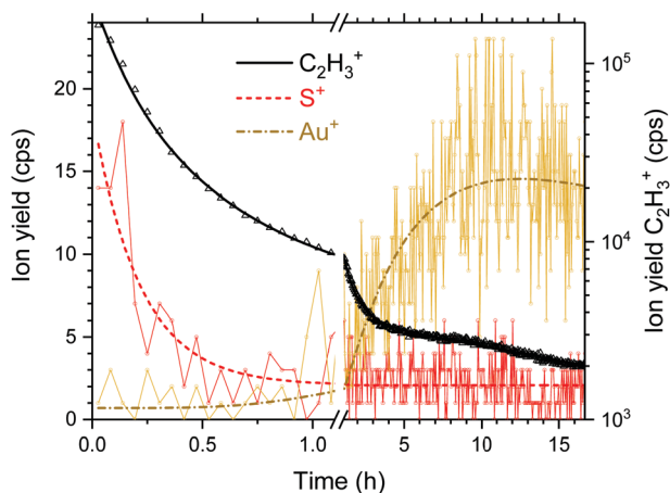
Fig. 3 Temporal evolution of the fragment ions \text{S}^+ and \text{C}_2\text{H}_3^+ of propanethiol and sputtered \text{Au}^+ from the Au(111) substrate upon long-term \text{Ar}^+ irradiation at 69 eV and 1.4 nA.
