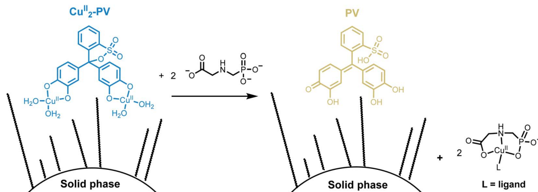
Fig. 2 Schematic representation of detection of GlyP with an immobilized \text{Cu}^{II}\text{-PV} complex by an indicator displacement assay using solid phase extraction.
