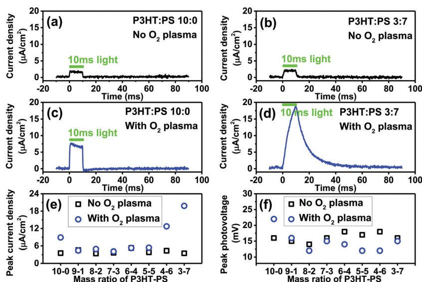
Fig. 7 Electrophotoreponse (EPR) measurements establish the photocurrent and photovoltage generated by an unbiased ITO/P3HT sample. 10 ms pulses of 515 nm light (50 mW cm -2 ) were used. (a) Example trace for a 10-0, untreated neat P3HT, photocurrent density. (b) P3HT-PS 3-7, untreated, photocurrent density. (c) 10-0, O 2 -plasma treated P3HT, photocurrent density. (d) 3-7, O 2 -plasma treated P3HT, photocurrent density. (e) Peak photocurrent density for the series of structured samples, comparing with and without plasma treatment. (f) Peak photovoltage for the series of structured samples, comparing with and without plasma treatment.
