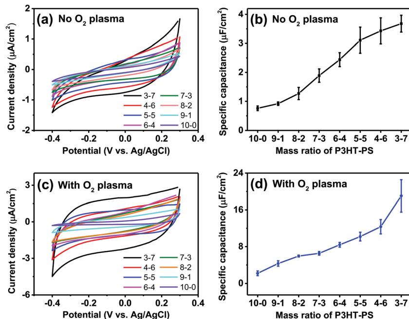
Fig. 6 Electrochemical capacitance evaluation of the structured P3HT films. (a) CV scans (100 mV s -1 ) of the P3HT films in the electrochemically-passive region of P3HT. (b) Average \pm SD of capacitance in \mu\text{F cm}^{-2} for different P3HT-PS mixing ratios, versus planar. (c) CV scans (100 mV s -1 ) of the O 2 plasma-treated P3HT. (d) Calculated capacitance values for plasma-treated samples.
