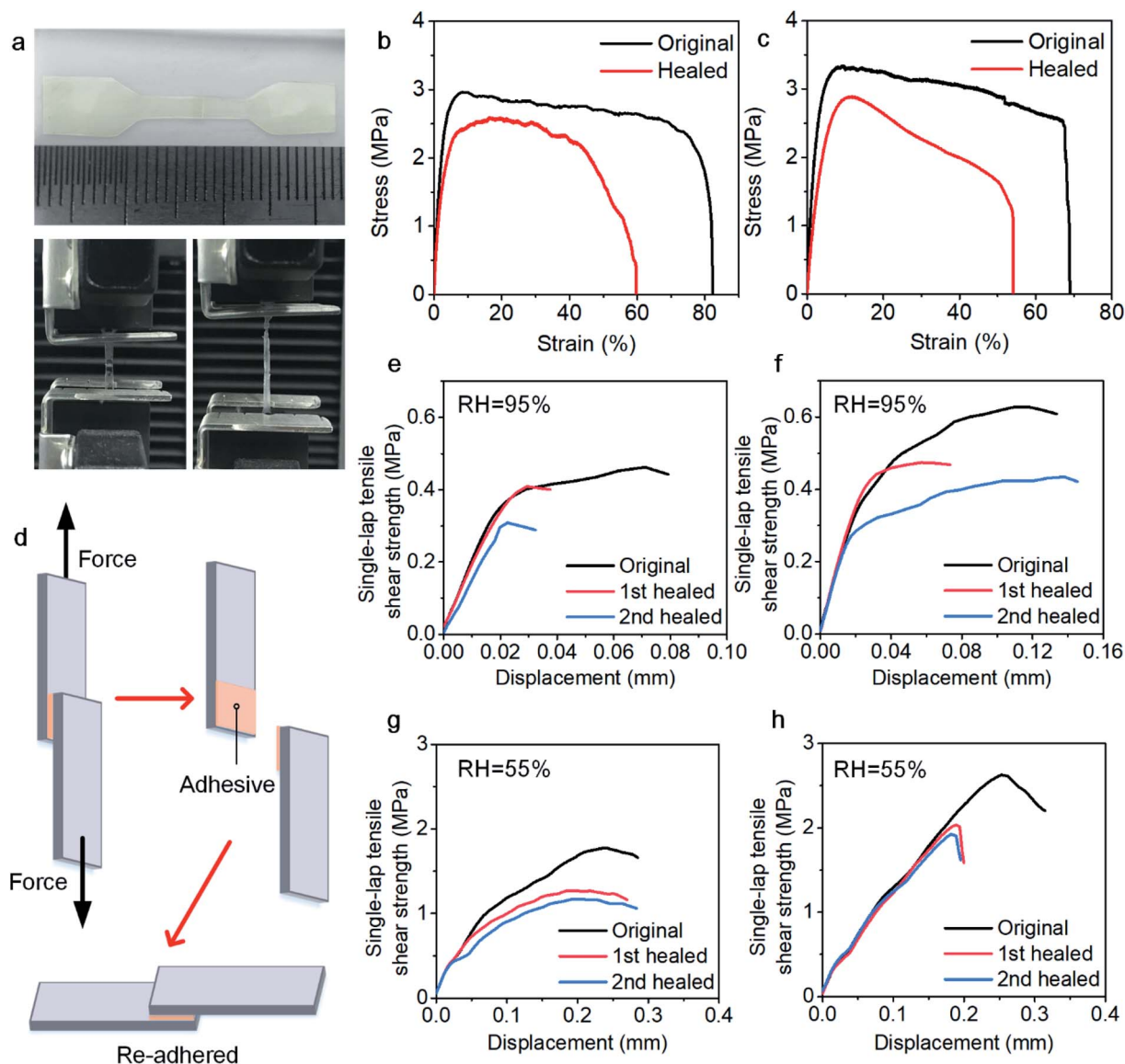
Fig. 2 Self-healing efficiency test. (a) Samples were cut and overlapped \sim 1 mm at \text{RH} \approx 95\% for 5 h, and the tensile tests were carried out in an ambient environment. The tensile stress-strain curve of (b) 30PHS/PEOZ and (c) 30PHS/PEOZ + \text{CaCl}_2 at \text{RH} \approx 95\% . (d) Scheme of the single-lap tensile shear strength test and repeatable adhesion. The repeatable adhesion strength of (e) 30PHS/PEOZ at \text{RH} \approx 95\% , (f) 30PHS/PEOZ + \text{CaCl}_2 at \text{RH} \approx 95\% , and (g) 30PHS/PEOZ at \text{RH} \approx 55\% , (h) 30PHS/PEOZ + \text{CaCl}_2 at \text{RH} \approx 55\% .
