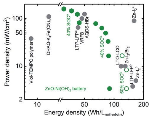
Fig. 6 Ragone plot of static semi-solid battery (Zn– \text{Ni}(\text{OH})_2 ) and reported redox flow battery chemistry including Viol–TEMPO polymer, 65 DHAQ– \text{K}_4\text{Fe}(\text{CN})_6 , 14 AQDS–HBr, 9 LTO–LCO, 26 LTP–LFP a,4 , LTP–LFP b,62 , VRFB, 12 Zn– \text{I}_2 /Br 2 , 35 Zn– \text{I}_2 a,38 and Zn– \text{I}_2 b,61 . The Zn–Ni semi-solid battery chemistry shown from this work contains anolyte with 5.2 vol% ZnO and catholyte with 7.6 (green hexagon, 40% SOC a ) and 12.5 vol% \text{Ni}(\text{OH})_2 (green solid 40% SOC b and open circles 60% SOC b ). Abbreviations: AQDS: 9,10-anthraquinone-2,7-disulphonic acid, DHAQ: 2,6-dihydroxyanthraquinone, TEMPO: 2,2,6,6-tetramethylpiperidinyloxy, Viol: viologen, LTP: \text{LiTi}_2(\text{PO}_4)_3 , LFP: \text{LiFePO}_4 , LTO: \text{Li}_4\text{Ti}_5\text{O}_{12} .
