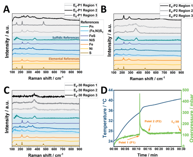
Fig. 5 Raman spectra of the obtained \text{E}_8\text{-Y} samples at three different time points of the mechanochemical reaction: closely before the initiation of the MSR reaction (A), closely after (B) and after 30 min of milling (C). The respective points are also shown for clarity in (D).
