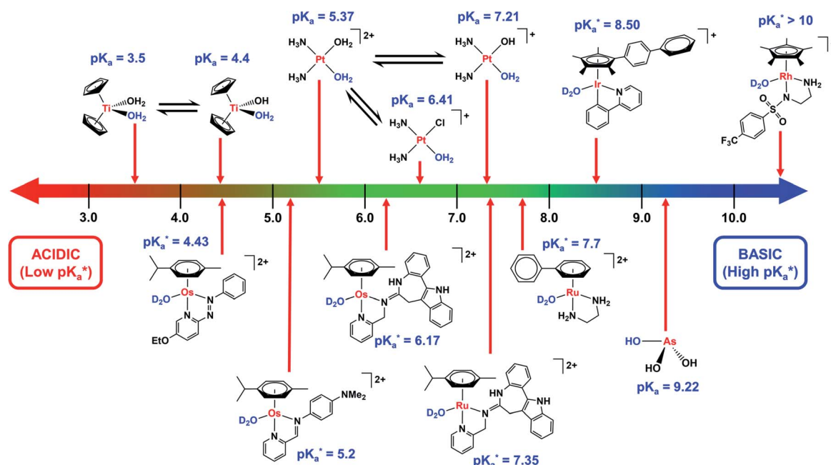
Fig. 3 Comparison of the \text{pK}_a values of aquated species of metal-based complexes. \text{pK}_a^* values refer to \text{M}-\text{OD}_2 complexes based on \text{pH}^* (pH meter reading not corrected for the effect of deuterium on the electrode).
