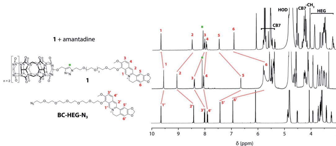
Fig. 3 Overlay of ^1\text{H} NMR (500 MHz, \text{D}_2\text{O} ) spectra of BC-HEG- \text{N}_3 (bottom), chemosensor 1 (middle) and chemosensor 1 with one equivalent of amantidine (top).
