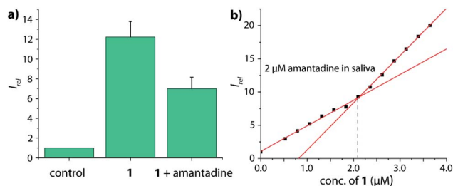
Fig. 8 (a) Normalized emission intensity at 540 nm of 5 \mu\text{M} chemo-sensor 1 in human saliva prior and after addition of 5 \mu\text{M} amantadine. Error bars represent the standard deviation of the mean ( n = 3 ). (b) Fitting plot of the normalized emission intensity at 540 nm obtained by the stepwise addition of 1 to saliva that was spiked with 2 \mu\text{M} amantadine, see the ESI† for repetition experiments and controls.
