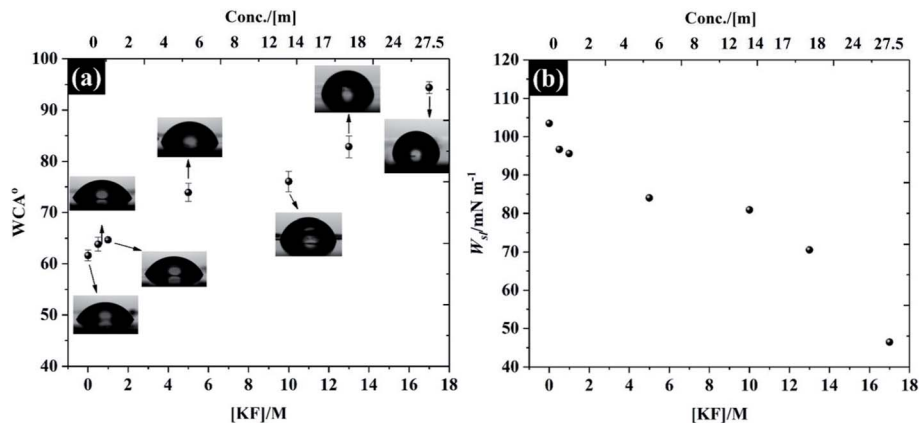
Fig. 8 Wettability of freshly cleaved highly ordered pyrolytic graphite (a) water in air contact angle at t = 0 s, and (b) work of adhesion as a function of KF concentration.
