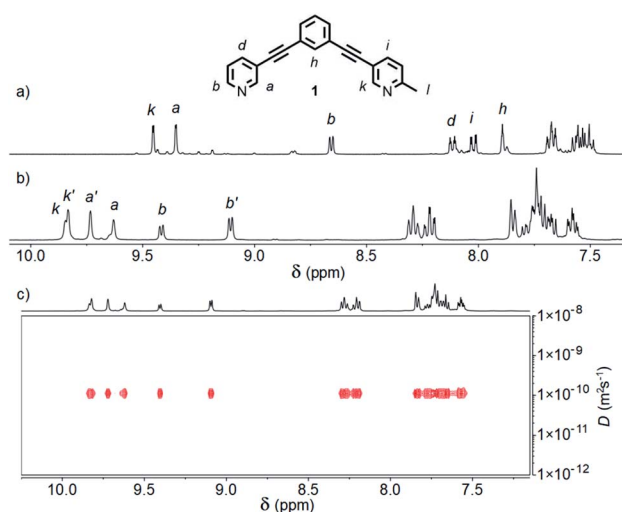
Fig. 2 Partial ^1\text{H} NMR spectra (400 MHz, 298 K) of cages [\text{Pd}_2(\text{1})_4](\text{BF}_4)_4 formed in (a) \text{CD}_3\text{CN} , and (b) d_6 -DMSO; (c) ^1\text{H} DOSY spectrum (500 MHz, d_6 -DMSO) of cis - and trans - [\text{Pd}_2(\text{1})_4](\text{BF}_4)_4 cage mixture.
