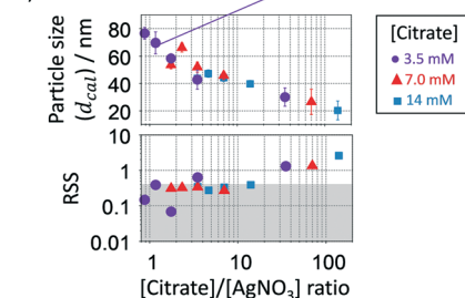
Fig. 10 Effect of the [citrate]/[ \text{AgNO}_3 ] ratio of the sequential additions in the growth-stage. A. UV-vis spectra, peak location and optical density of particles in R5. B. Calculated average particle size and spherical degree (RSS) using the Mie theory-based algorithm. For smaller particle sizes, the number of growth reactors should be reduced. Conditions: nucleation reactor \rightarrow refer to Fig. 5 growth reactors \rightarrow same as Fig. 6 and 7 except for changes in the citrate/ \text{AgNO}_3 ratio.
