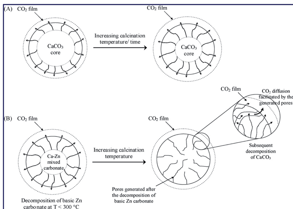
Scheme 3 Proposed models for \text{CaCO}_3 decomposition to \text{CaO} (A) and mixed precipitate of \text{Ca} – \text{Zn} (B). Reproduced from ref. 150.
