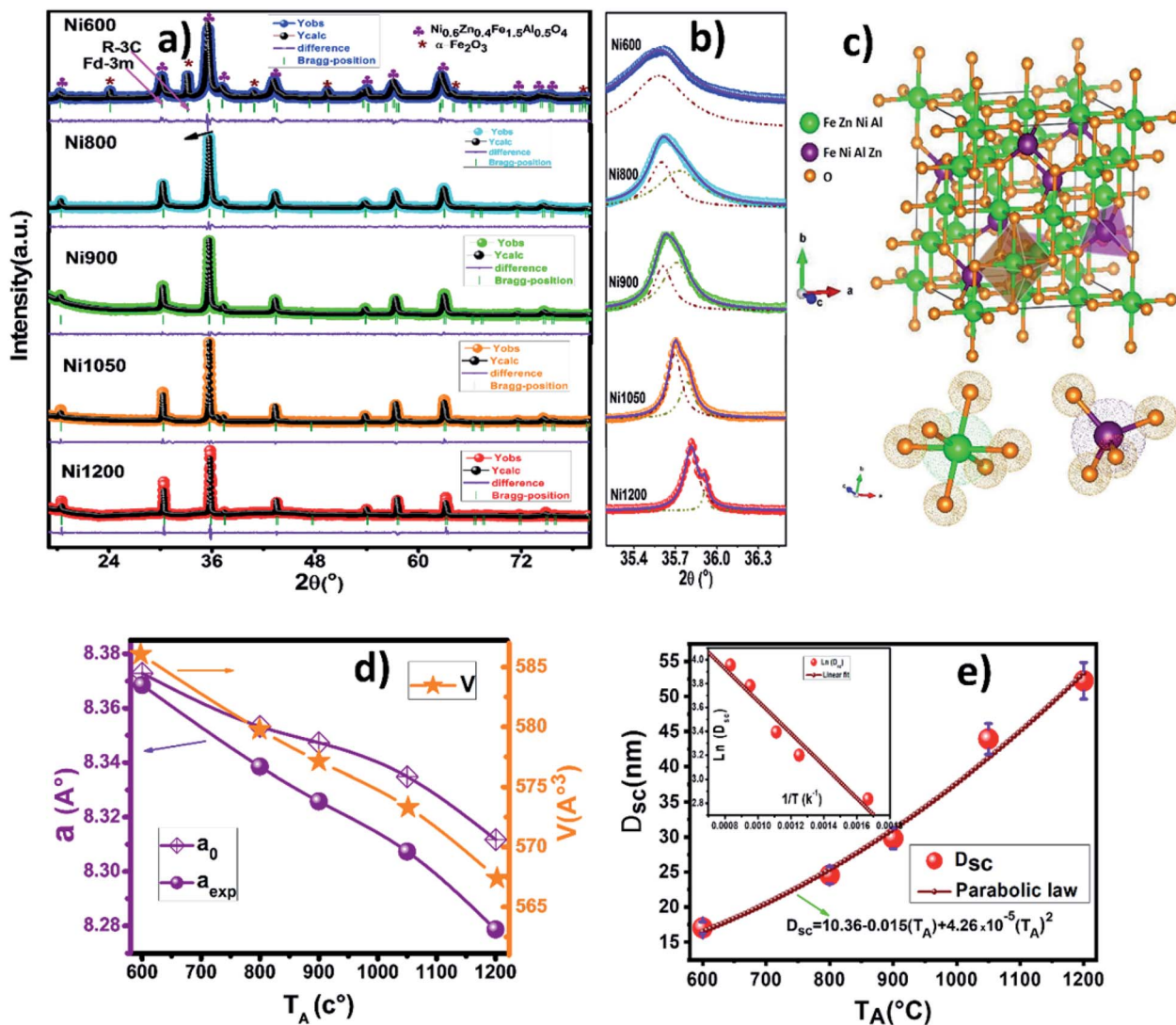
Fig. 3 (a) Rietveld refined X-ray diffraction patterns of Ni_{0.6}Zn_{0.4}Al_{0.5}Fe_{1.5}O_4 annealed at 600, 800, 900, 1050 and 1200 °C. (b) Zoomed views in the 2\theta interval of 35.1–36.3°. (c) Unit cell of the sample showing the tetrahedral (A) and octahedral (B) sites. (d) Lattice parameters and volume of the ferrites compounds against annealing temperature. (e) D_{sc} versus the annealing temperature T_A , where the solid line shows the fit to the parabolic law and the fitted values are shown.
