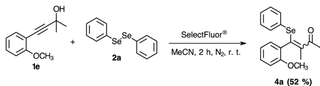
Scheme 4 Reactivity of 2-propagylanisole 1e in the reaction with the electrophilic Se–F species.
