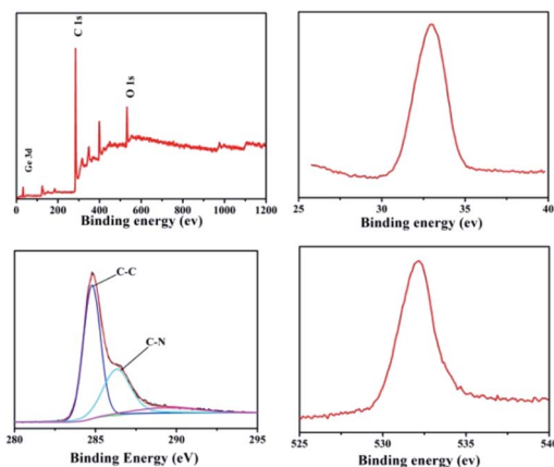
Fig. 2 XPS spectra of \text{GeO}_2/\text{nanocable} : (a) the full XPS spectrum of the \text{GeO}_2/\text{nanocable} ; (b–d) high-resolution spectra Ge 3d, C 1s and O 1s, respectively.
