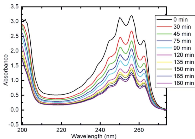
Fig. 9 UV-visible spectra of pyridine showing its degradation with time (10 mg of nanocomposite, 50 ml Py solution (100 ppm), 25^\circ\text{C} and pH 7).
