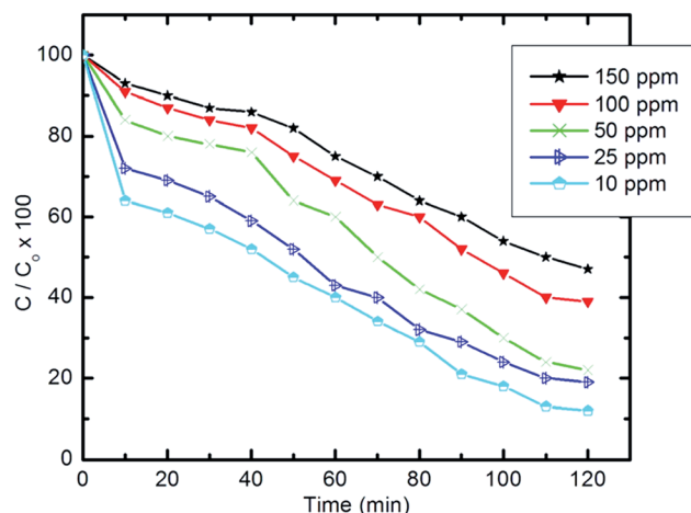
Fig. 10 Effect of initial concentration of pyridine solution on the degradation efficiency (10 mg of composite, 50 ml Py solution, 25^\circ\text{C} and pH 7).
