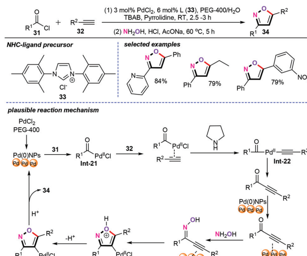
Scheme 16 PdNP-catalyzed regioselective one-pot synthesis of isoxazoles in PEG-400.
