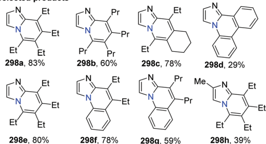
Scheme 71 Tandem synthesis of substituted azolopyridines catalyzed by CuI.
