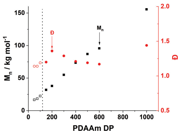
Fig. 9 Evolution of molar mass and dispersity versus PDAAm DP ( y ) for a series of PDMAM 46 - b -PDAAm y polymers synthesised in the flow reactor with respect to increasing PDAAm DP. The residence time was set to 20 minutes and reactions were performed at either 70 °C (filled) or 90 °C (hollow). Reaction solution were made at 20% w/w total final solids and adjusted to pH 3.
