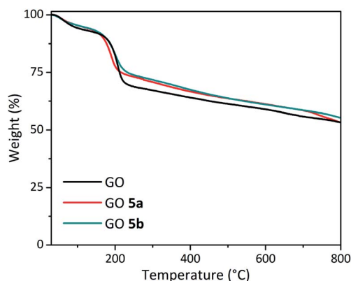
Fig. 5 TGA of the pristine GO, GO 5a and GO 5b performed in an inert atmosphere.
