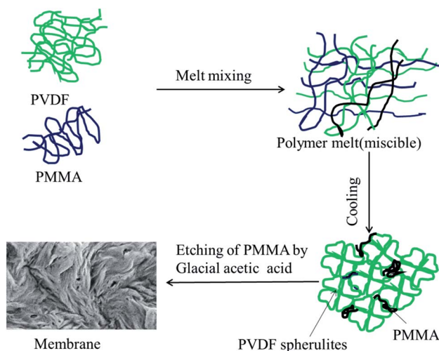
Fig. 1 Schematic representation of the membrane fabrication by crystallization induced phase separation.
