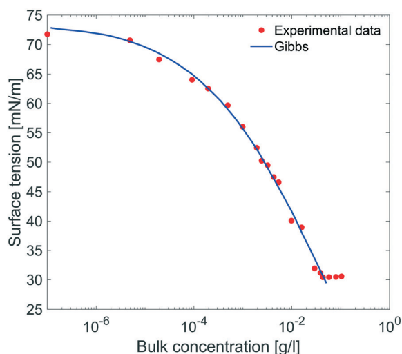
Fig. 9 Equilibrium surface tension from Fig. 8 as a function of bulk concentration and compared with the results obtained using the Gibbs adsorption eqn (4).
