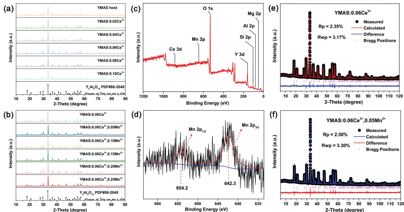
Fig. 1 XRD patterns of YMAS: x\text{Ce}^{3+} ( x = 0\text{--}0.10 ) (a) and YMAS: 0.06\text{Ce}^{3+}, y\text{Mn}^{2+} ( y = 0\text{--}0.25 ) (b) with the standard of \text{Y}_3\text{Al}_5\text{O}_{12} (PDF #88-2048). The XPS survey spectrum (c) and high-resolution spectrum (d) of YMAS: 0.06\text{Ce}^{3+}, 0.25\text{Mn}^{2+} . Rietveld refinement results of YMAS: 0.06\text{Ce}^{3+} (e) and YMAS: 0.06\text{Ce}^{3+}, 0.05\text{Mn}^{2+} (f).
