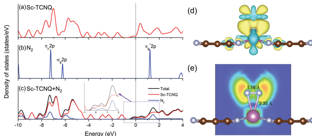
Fig. 4 Density of states of (a) pristine Sc-TCNQ, (b) \text{N}_2 molecule in the gas phase, and (c) Sc-TCNQ with one adsorbed \text{N}_2 molecule. Fermi level is set to zero and denoted in the black line. Inset in (c) shows the zoomed DOS near the Fermi level. (d) Charge density difference distribution (charge accumulation and depletion are shown in yellow and light blue, respectively) of \text{N}_2 adsorption with the side-on configuration, and (e) corresponding ELF map with bond lengths of Sc–N and N–N marked in the figure.
