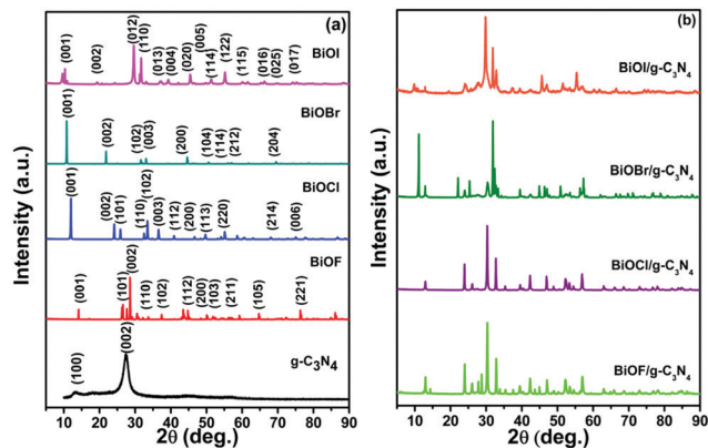
Fig. 1 PXRD pattern of (a) \text{g-C}_3\text{N}_4 , \text{BiOX} ( \text{X} = \text{F}, \text{Cl}, \text{Br} and \text{I} ) and (b) \text{BiOX}/\text{g-C}_3\text{N}_4 composites.
