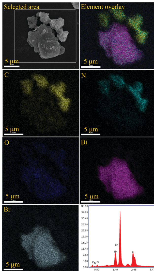
Fig. 5 Elemental mapping and EDAX spectrum of the \text{BiOBr}/\text{g-C}_3\text{N}_4 composite.
