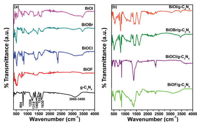
Fig. 2 FTIR spectra of (a) \text{g-C}_3\text{N}_4 , \text{BiOX} ( \text{X} = \text{F}, \text{Cl}, \text{Br} and \text{I} ) and (b) \text{BiOX}/\text{g-C}_3\text{N}_4 composites.
