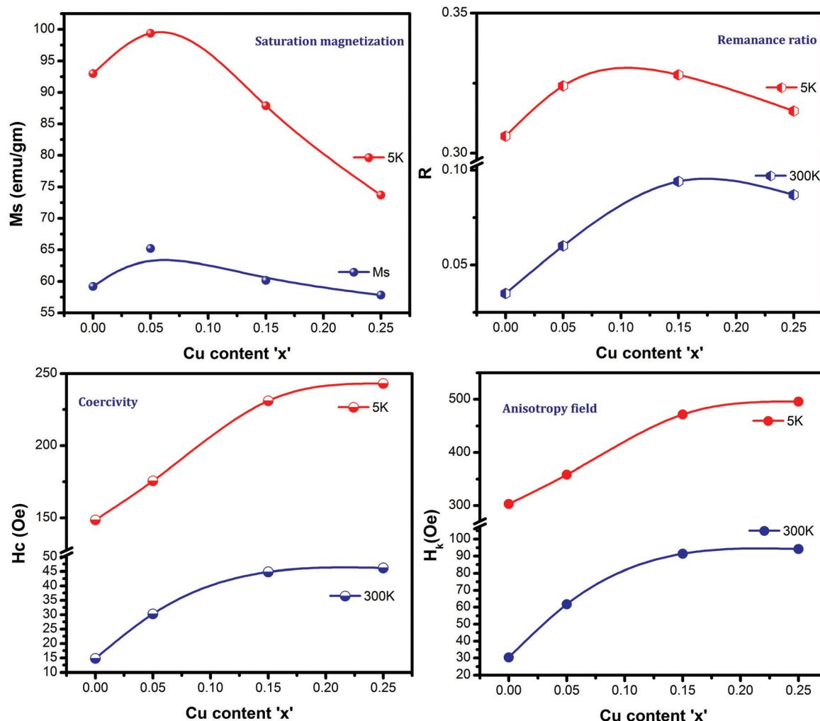
Fig. 9 Magnetic parameters for \text{Ni}_{0.70-x}\text{Cu}_{0.30}\text{Zn}_{0.30}\text{Fe}_2\text{O}_4 ( x = 0.00, 0.05, 0.15 , and 0.25 ) at 300 K and 5 K.
