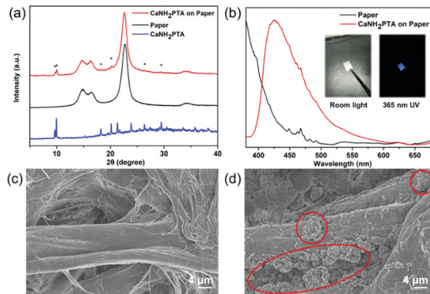
Fig. 5 Preparation of the luminescent test paper: (a) PXRD patterns of the as-made paper loaded with \text{CaNH}_2\text{PTA} (ROD-95; asterisks represent the peaks of MOF); (b) emission spectra of fluorescent and bare paper (insets show the test paper under room light and 365 nm UV light) and (c and d) SEM images of the substrate without and with MOF loading (red circles indicate the growth of MOF particles on paper fibres).
