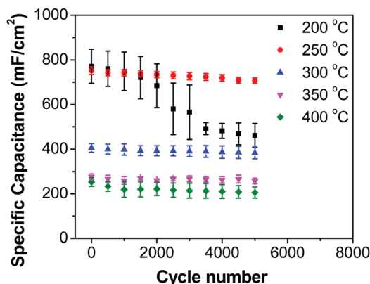
Fig. 15 Specific capacitances at different GCD cycle numbers for various \text{RuO}_2 -CNF electrodes measured at 200 \text{ mA}/\text{cm}^2 .
