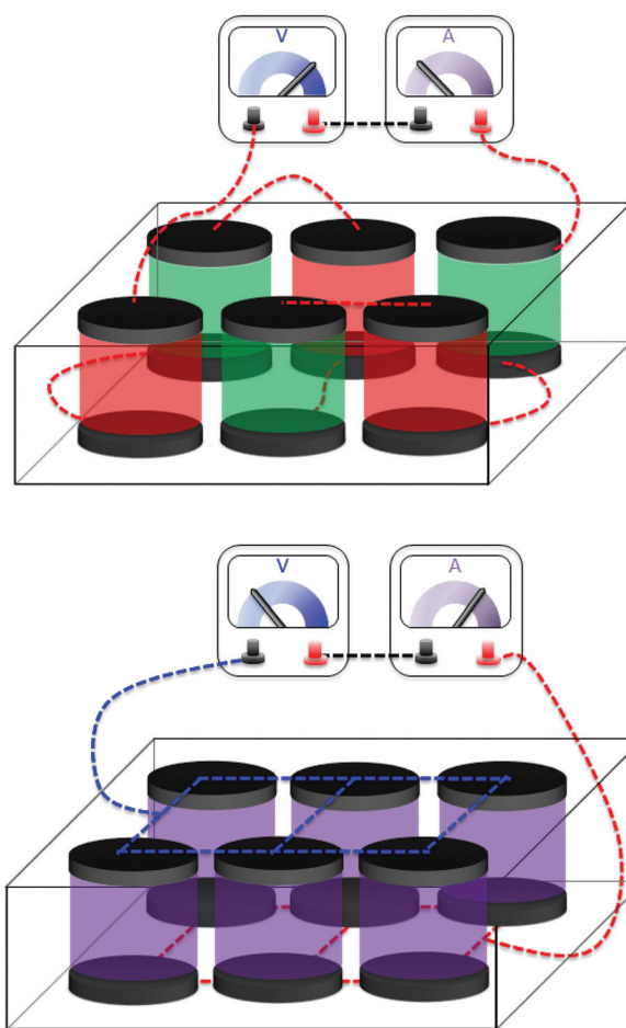
Fig. 10 Showing power curves (filled symbols; solid lines) and I - V data (hollow symbols; dashed lines), as well as associated schematic cartoons, for (a) one pair of [\text{Fe}(\text{HSO}_4)]^{+/2+} – [\text{Fe}(\text{SO}_4)_2]^{-/2-} thermocells electrically in-series (black diamonds) and three pairs in-series (black inverted triangles). Similar data is shown in (b) after the two electrolytes have been mixed, showing the data for one mixed electrolyte thermocell (purple diamonds) and six mixed electrolyte thermocells electrically in-parallel (purple triangles). All measurements recorded at an applied \Delta T of 20 K ( T_c = 20^\circ\text{C} ).
