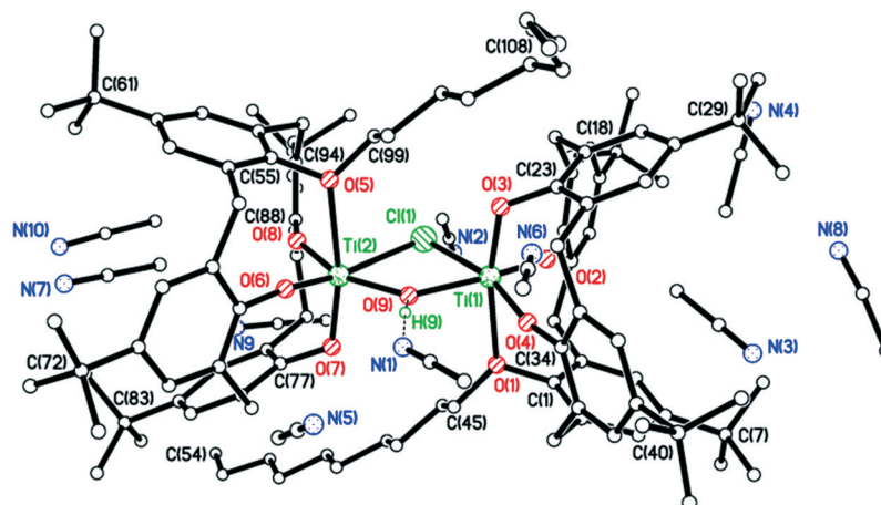
Fig. 7 Molecular structure of \{[TiL(O)_3(On-decyl)]_2(\mu-Cl)(\mu-OH)\} \cdot 8.5MeCN (10·8.5MeCN) (most H atoms are omitted for clarity). Selected bond lengths (Å) and angles (°): Ti(1)–O(1) 2.381(3), Ti(1)–O(2) 1.817(3), Ti(1)–O(3) 1.852(3), Ti(1)–O(4) 1.793(3), Ti(1)–O(9) 2.000(3), Ti(1)–Cl(1) 2.5177(14); O(1)–Ti(1)–O(3) 168.54(13), O(2)–Ti(1)–O(4) 102.84(15), Cl(1)–Ti(1)–O(9) 74.82(10), Ti(1)–O(1)–C(1) 112.8(2), Ti(1)–O(2)–C(12) 150.5(3), Ti(1)–O(3)–C(23) 119.9(2), Ti(1)–O(4)–C(34) 168.3(3).
