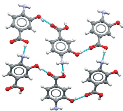
Fig. 2 Hydrogen bonding observed in the crystal structure of 4-amino-3-hydroxyl-benzoic acid (3-OH- p AABA).
