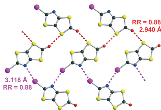
Fig. 1 Detail of the I...N XB (pink dotted line) and S...O ChB (red dotted line) interactions in 2 .
