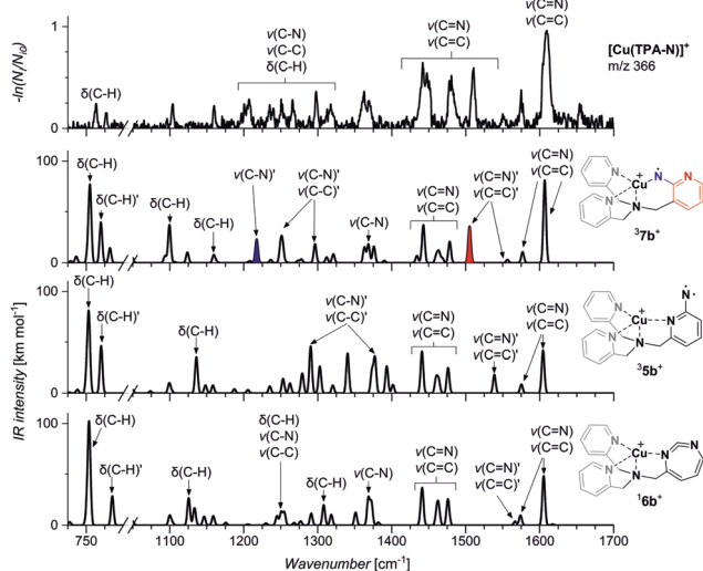
Fig. 3 Helium tagging infrared photodissociation spectrum of [\text{Cu}(\text{TPA-N})]^+ ( m/z 366) (top panel). Theoretical IR spectra of 7b , 5b and 6b were calculated for the optimized structures at the B3LYP/6-31+G* level and scaled by 0.97. \delta(\text{C-H}) , \nu(\text{C=C}) and \nu(\text{C=N}) correspond to the absorption bands in the pyridine rings whereas \delta(\text{C-H})' , \nu(\text{C=C})' and \nu(\text{C=N})' correspond to the absorption bands in the nitrene-pyridine ring.
