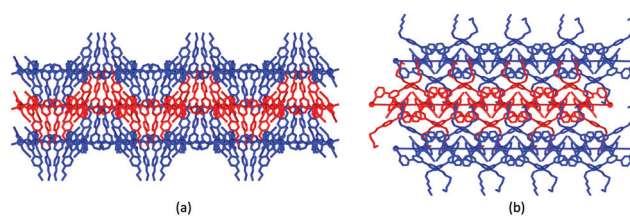
Fig. 3 Packing of (4,4) nets in (a) [\text{Co}(\text{NCS})_2\{4'-(4\text{-EtOC}_6\text{H}_4)-3,2':6',3''\text{-tpy}\}_2]_n (CSD refcode OHESAY) and (b) [\text{Co}(\text{NCS})_2\{4'-(4\text{-}^n\text{HxOC}_6\text{H}_4)-3,2':6',3''\text{-tpy}\}_2]_n (CSD refcode OHESEC). H atoms omitted.
