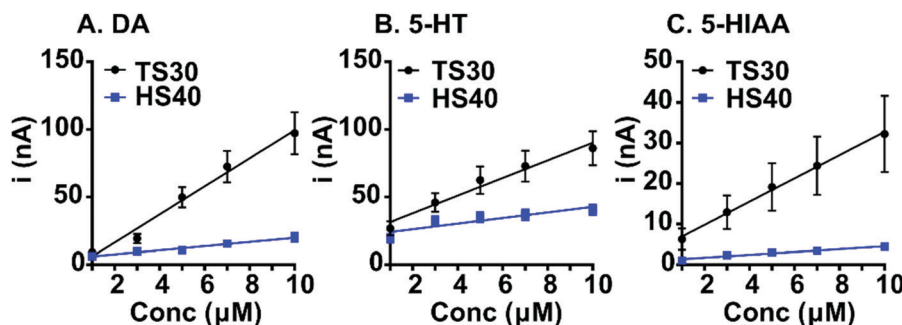
Fig. 3 Sensitivity comparison for TS30 and HS40 fibers. All calibration curves were conducted from 1 \mu\text{M} to 10 \mu\text{M} . (A) Dopamine (waveform: -0.4 V to 1.3 V, 400 V \text{s}^{-1} , n = 6-10 ), (B) 5-HT, and (C) 5-HIAA (waveform for TS30: 0.2 V to 1.0 V, down to -0.1 V and back to 0.2 V, 1000 V \text{s}^{-1} ; HS40: -0.4 V to 1.3 V, 400 V \text{s}^{-1} , n = 8-10 ).
