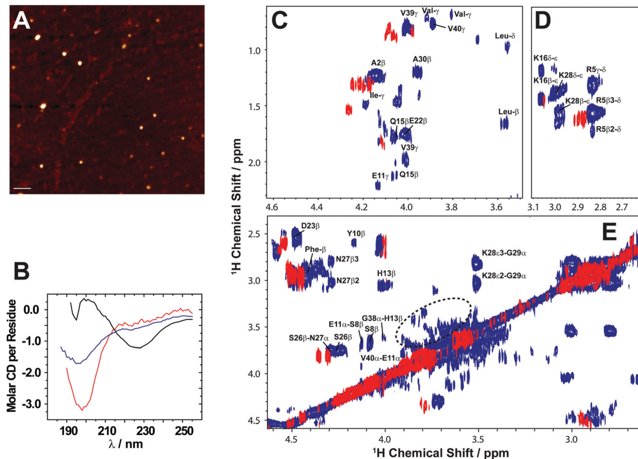
Fig. 3 Solid state NMR allows characterization of growing low abundance A\beta_{1-40} oligomers. (A) AFM image showing the presence of A\beta_{1-40} oligomers after separation from fibers after 4 days (scale bar is 100 nm). (B) CD spectra show that the filtered A\beta_{1-40} oligomers (blue) are disordered, similar to the freshly dissolved monomers (red), and differ from the \beta -sheet rich fibers (black). (C–E) 2D ^1H/^1H NMR spectra obtained via RFDR recoupling of ^1H-^1H dipolar couplings show high-resolution cross-peaks for oligomers (blue) and freshly dissolved A\beta_{1-40} monomers (red); spectra recorded at 25 °C under 2.7 kHz MAS on a 600 MHz solid-state NMR spectrometer. The spectrum highlights the observation of cross-peaks due to the recoupled ^1H-^1H dipolar couplings for (C) side-chain to H\alpha , (D) side-chain, and (E) H\beta-H\alpha and H\alpha-H\alpha regions. The acquisition time was 4 days. The 2.7 kHz MAS and RFDR mixing enabled the suppression of signals from monomers and fibers and selective observation of low molecular weight oligomers in a non-perturbative manner. The NMR samples were prepared in 10 mM phosphate buffer, pH 7.4, and 10% D_2O . Copyright © 2015, Springer Nature. This figure is reproduced from Scientific Reports: DOI: 10.1038/srep11811. Further details can be found in the referenced work. 103
